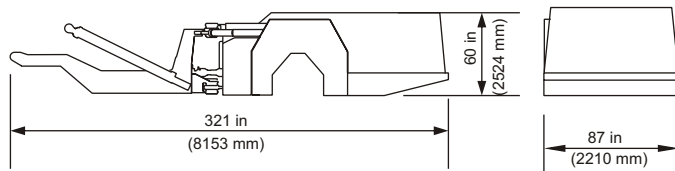
3. Dump box, cab, exhaust, axles and cradle removed Weight: 27030 lbs (12260 kg)
